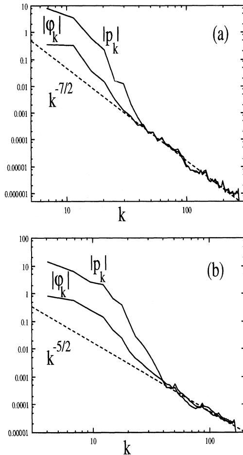
FIG. 4. Wave-number spectra of potential \varphi and density fluctuation p for (a) B = 1.5B_c (time-periodic case), and (b) B = 2.6B_c (time-chaotic state). Note that k is the averaged transverse wave number.
